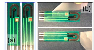
Prof. Mark Sheplak's complete sensor package for a flush-mounted, dual-axis differential capacitive wall shear stress sensor.
