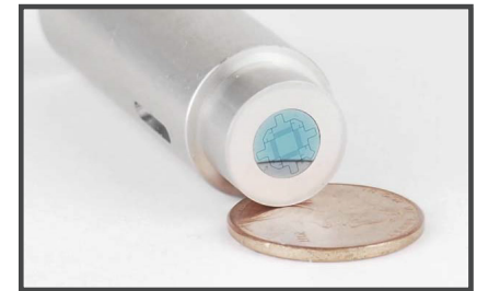
Prof. Mark Sheplak's complete sensor package for a flush-mounted, dual-axis differential capacitive wall shear stress sensor.
